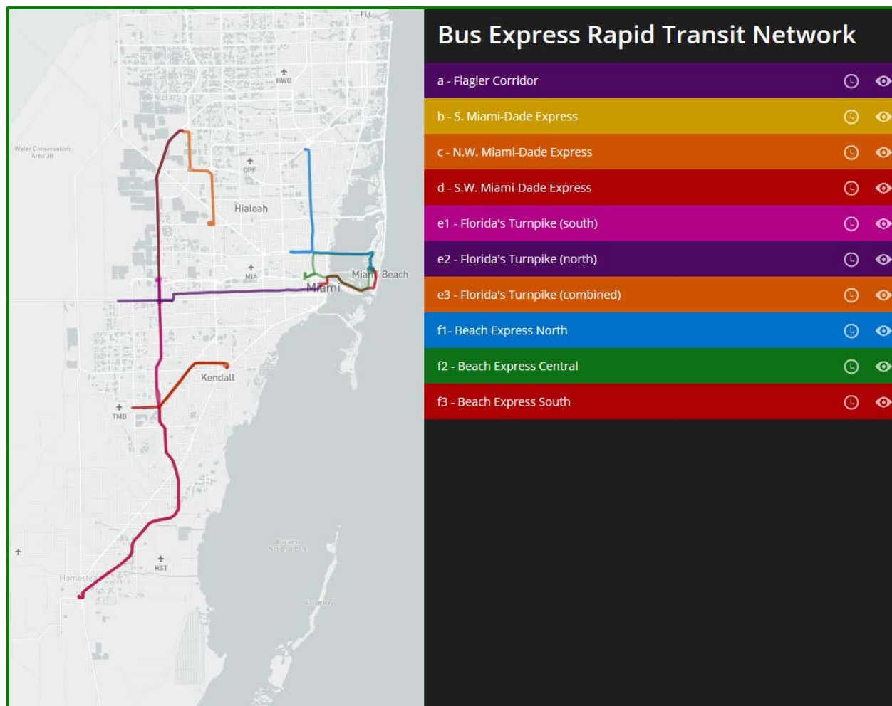
Figure 1 BERT Network
