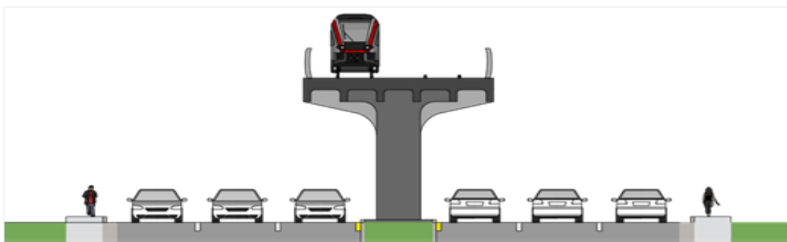
Elevated HRT (Metrorail) Typical Section
